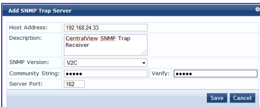
Figure 252: Add SNMP Trap Server
