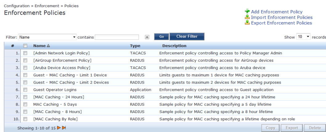
Figure 199: Enforcement Policies Listing Page
